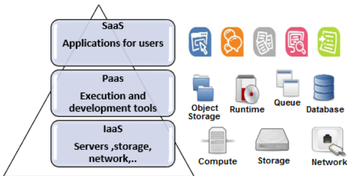
Figure 1: The Main Three Cloud Computing Layers
